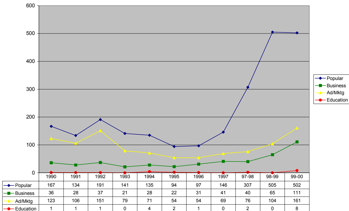
Graph 6: Electronic Marketing
